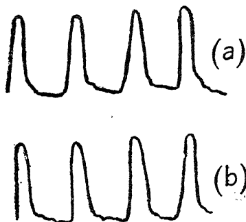
(a) Series of electric responses to successive mechanical stimuli at intervals of half a minute, in tin. (b) Mechanical responses in muscle.
